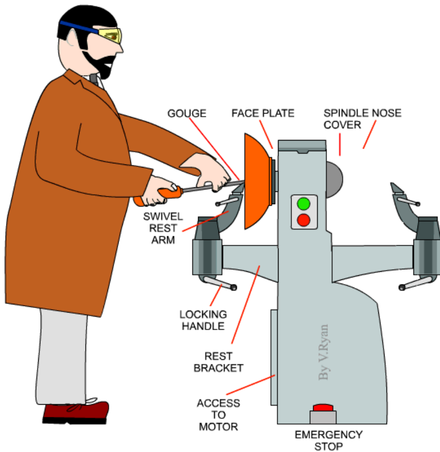
A SHORT BED WOODTURNING LATHE
